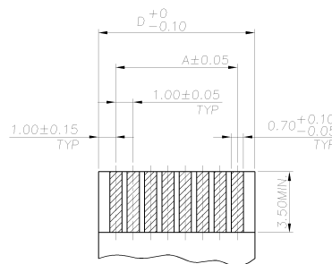
RECOMMENDED FPC/FFC LAYOUT (THICKNESS=0.30±0.05)
