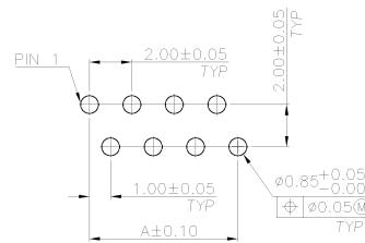
RECOMMENDED PCB LAYOUT TYPE B (THICKNESS=1.60)
