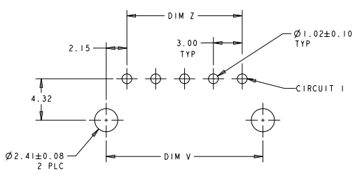
PCB LAYOUT COMPONENT SIDE
