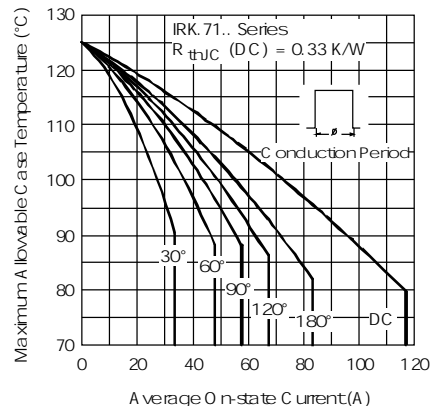
Fig. 38 - Current Ratings Characteristics
