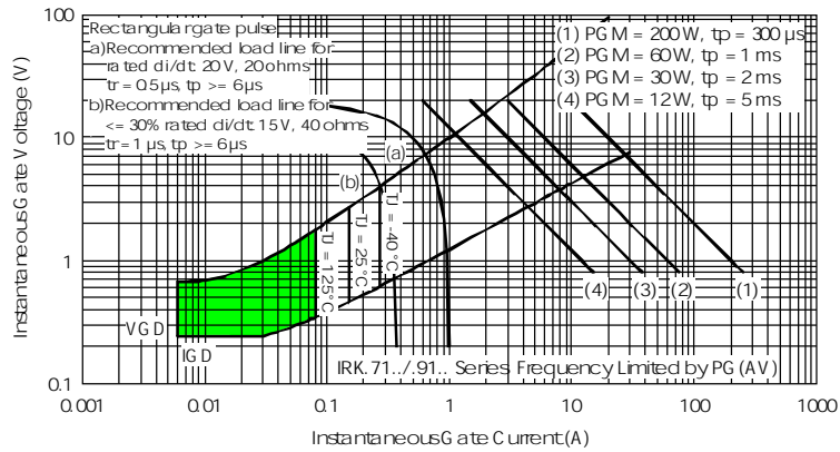
Fig. 60 - Gate Characteristics
