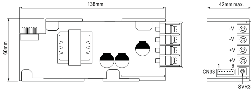
Output Connector(CN33) : JST B6B-XH or equivalent
