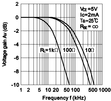
Fig.11 Frequency Response
