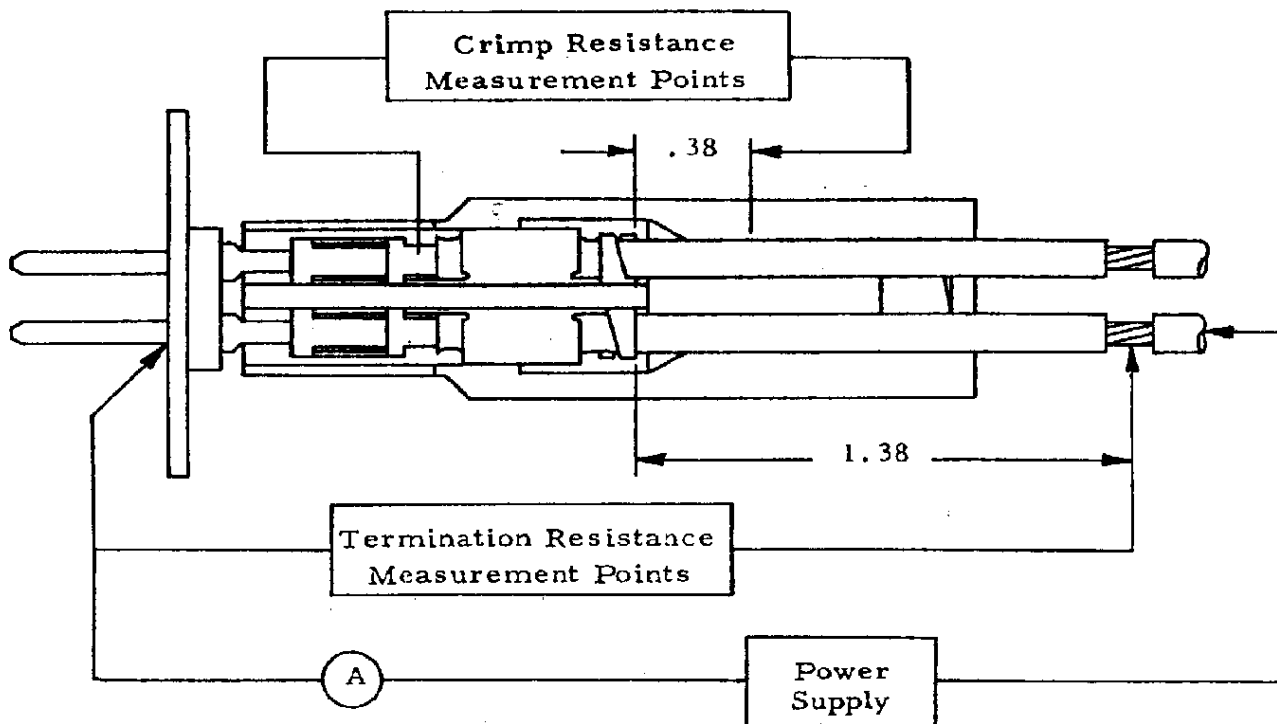
Figure 3 Resistance Measurement Points
