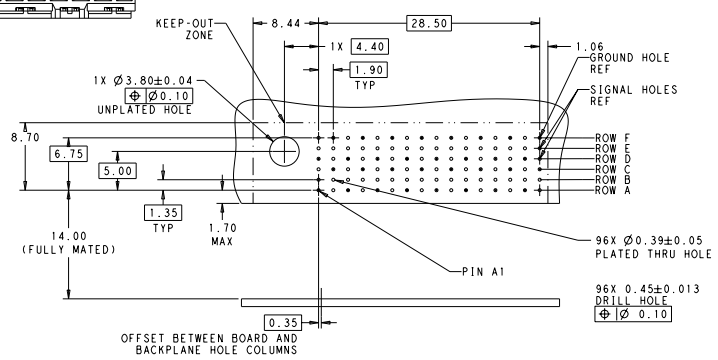
RECOMMENDED PCB LAYOUT MIN BOARD THICKNESS 1.6
