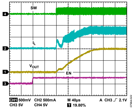
Figure 21. Startup, V_{OUT} = 1.0V , 600 mA
