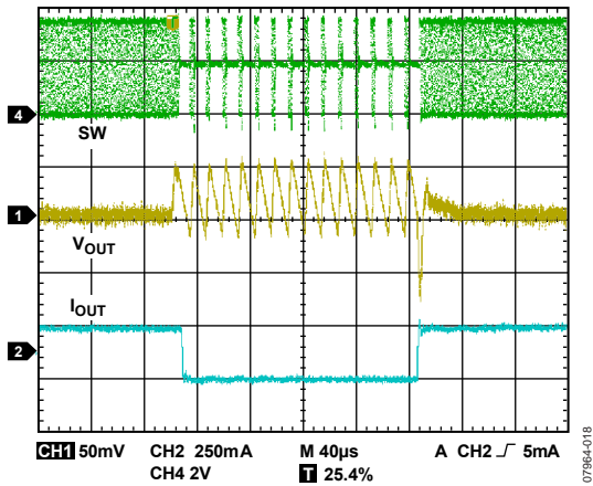
Figure 17. Load Transient, V_{OUT} = 1.8V , 50 mA to 300 mA
