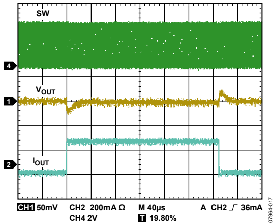
Figure 16. Load Transient, V_{OUT} = 1.8V , 300 mA to 600 mA
