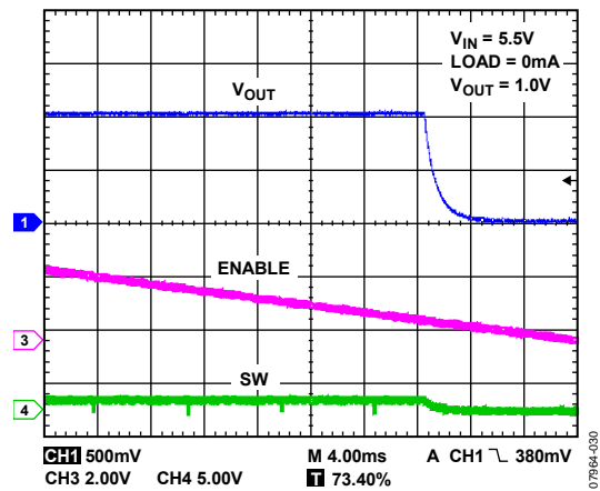
Figure 22. Typical Discharge Curve, V_{OUT} = 1.0V , V_{IN} = 5.5V
