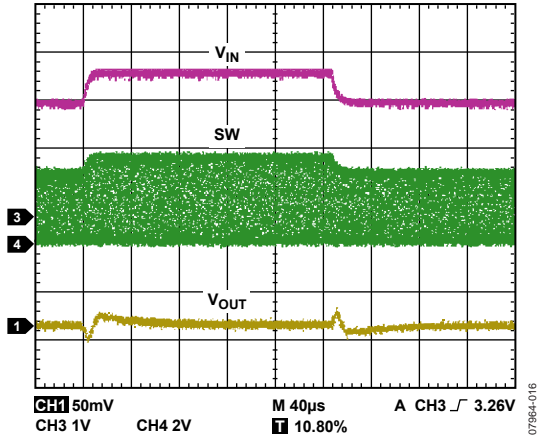
Figure 15. Line Transient, V_{OUT} = 1.0V
