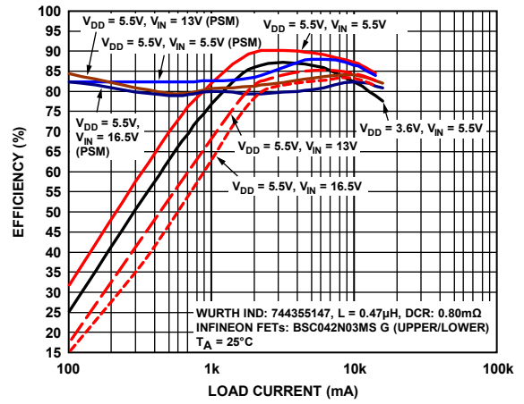
Figure 7. Efficiency—600 kHz, V_{OUT} = 0.8 V
