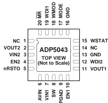
Figure 2. Pin Configuration
