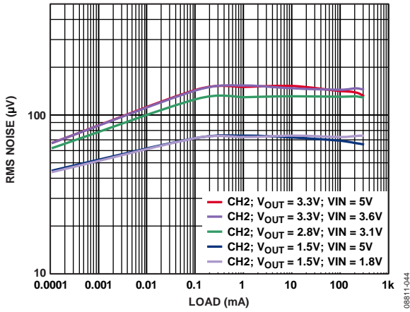
Figure 45. LDO1 Output Noise vs. Load Current, Across Input and Output Voltage
