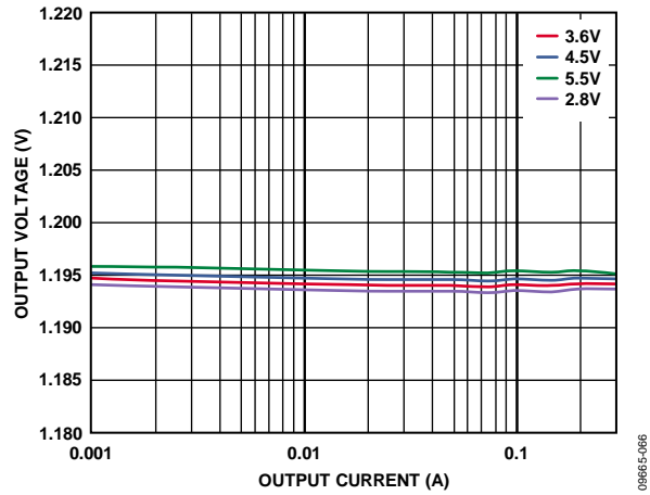
Figure 66. LDO1, LDO2 Load Regulation Across Input Voltage, V_{OUT} = 1.2 V
