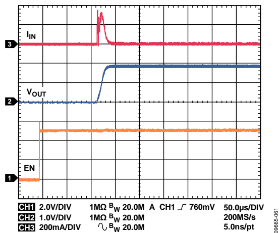
Figure 61. LDO1, LDO2 Startup, V_{OUT} = 1.8\text{ V} , I_{OUT} = 5\text{ mA}
