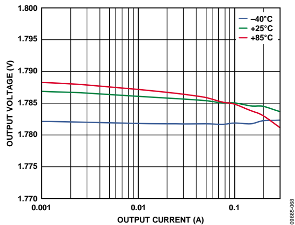
Figure 68. LDO1, LDO2 Load Regulation Across Temperature, V_{IN} = 3.6 V , V_{OUT} = 1.8 V
