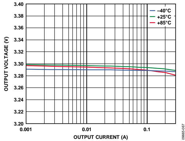
Figure 67. LDO1, LDO2 Load Regulation Across Temperature, V_{IN} = 3.6 V , V_{OUT} = 3.3 V
