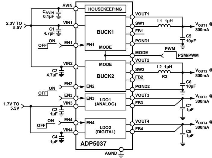
Figure 52. ADP5037 Fixed Output Voltages with Enable Pins
