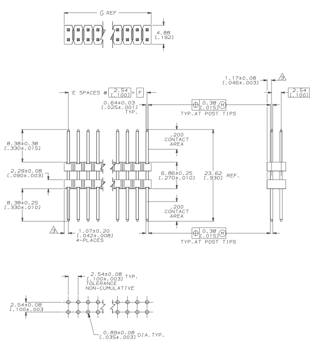
RECOMMENDED HOLE LAYOUT
