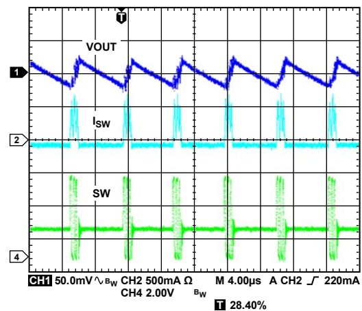
Figure 20. Typical Waveforms, V_{OUT2} = 1.8\text{ V} , I_{OUT2} = 30\text{ mA} , Auto Mode
