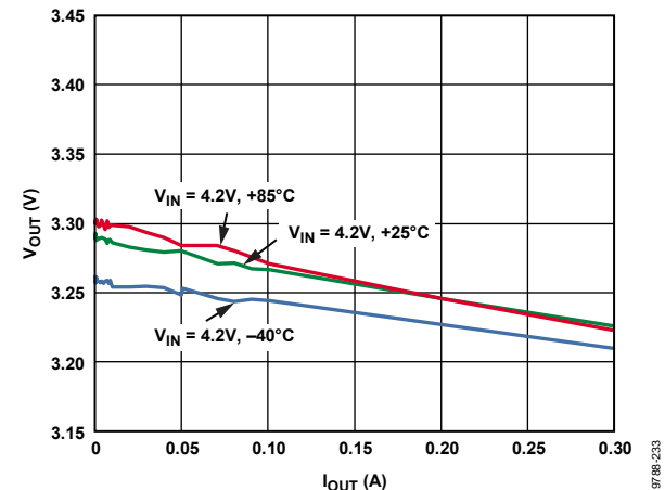
Figure 32. LDO Load Regulation Across Temperature, V_{IN3} = 4.2 V, V_{OUT3} = 3.3 V
