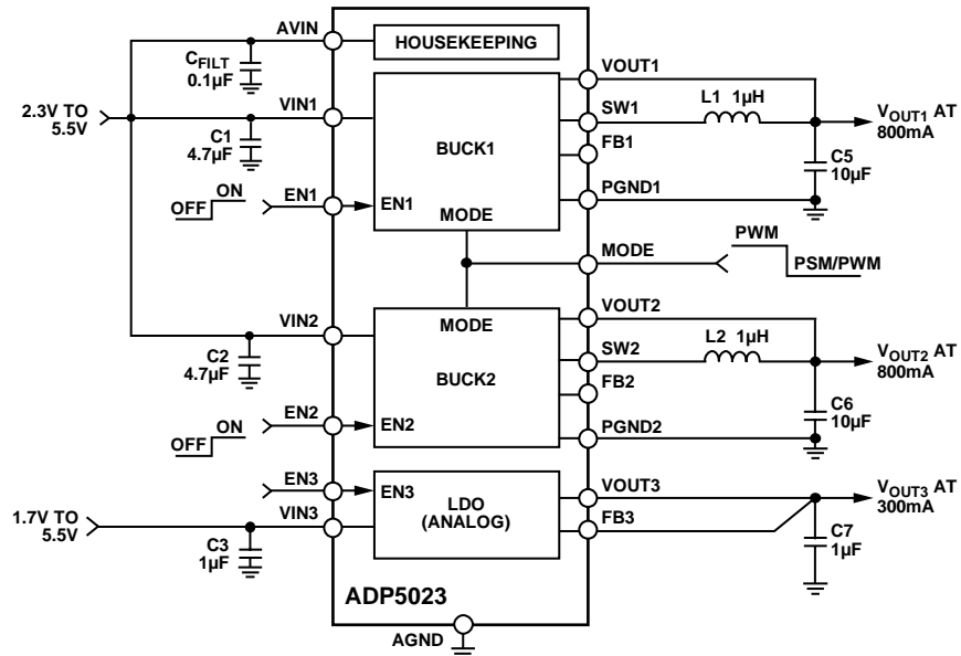
Figure 52. ADP5023 Fixed Output Voltages with Enable Pins
