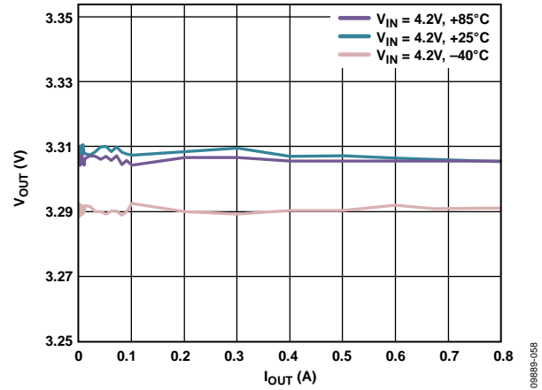
Figure 6. BUCK1 Load Regulation Across Temperature, V_{OUT1} = 3.3\text{ V} , Auto Mode
