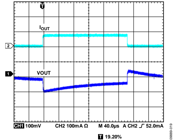
Figure 37. LDO Response to Load Transient, I_{OUT3} = 1\text{ mA} to 80\text{ mA} , V_{OUT3} = 2.8\text{ V}
