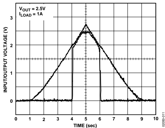
Figure 11. Power-Up/Power-Down
