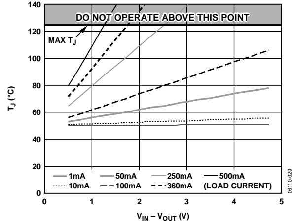
Figure 41. 0.00 mm 2 of PCB Copper, T A = 50°C
