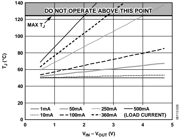
Figure 38. 0.70 mm 2 of PCB Copper, T A = 50°C
