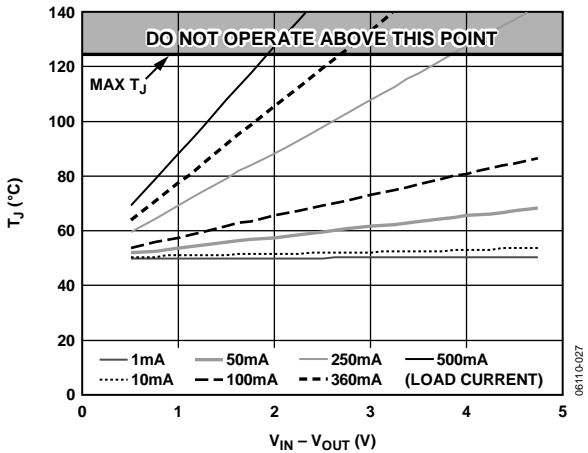
Figure 39. 0.30 mm 2 of PCB Copper, T A = 50°C
