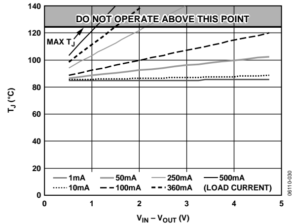
Figure 42. 0.70 mm 2 of PCB Copper, T A = 85°C
