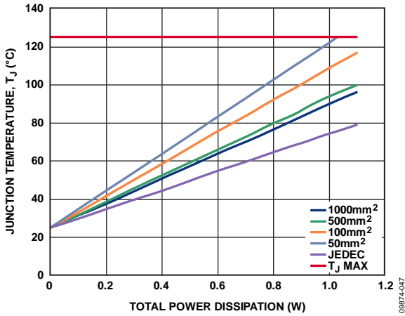
Figure 47. Junction Temperature vs. Total Power Dissipation, T_A = 25^\circ\text{C}
