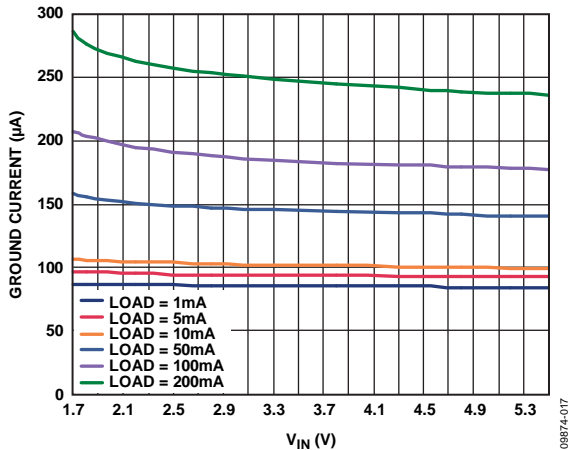
Figure 17. Ground Current vs. Input Voltage, All Outputs Loaded Equally
