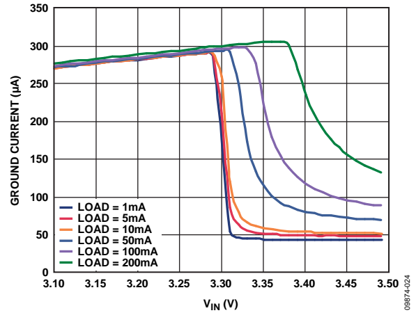
Figure 24. Ground Current vs. Input Voltage (in Dropout), V_{OUT1} = 3.3\text{ V}
