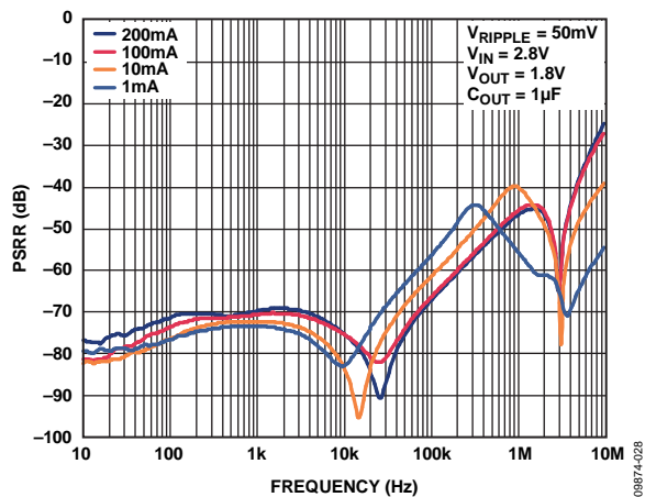
Figure 28. Power Supply Rejection Ratio vs. Frequency, 1.8 V
