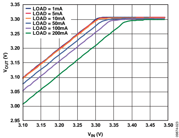
Figure 23. Output Voltage vs. Input Voltage (In Dropout), V_{OUT1} = 3.3\text{ V}
