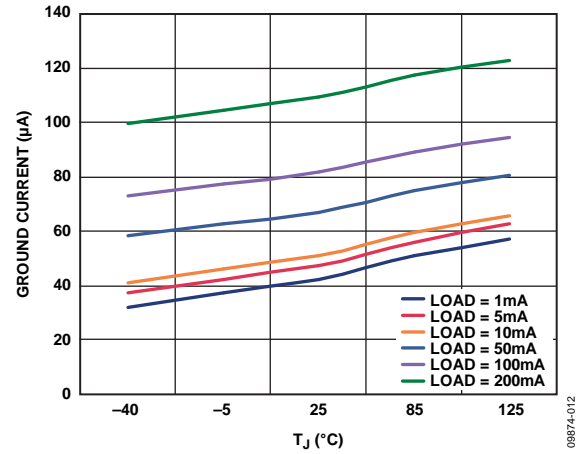
Figure 12. Ground Current vs. Junction Temperature, Single Output Loaded
