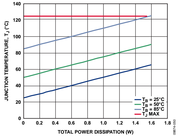
Figure 50. Junction Temperature vs. Total Power Dissipation and Board Temperature
