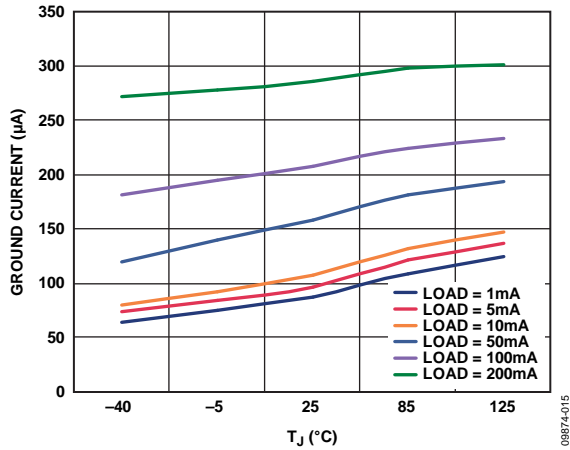
Figure 15. Ground Current vs. Junction Temperature, All Outputs Loaded Equally
