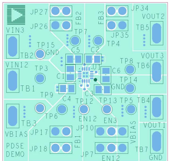
Figure 51. Example of PCB Layout, Top Side
