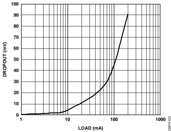
Figure 22. Dropout Voltage vs. Load Current and Output Voltage, V_{OUT1} = 3.3\text{ V}
