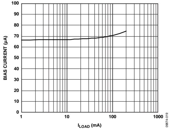
Figure 19. Bias Current vs. Load Current, Single Output Load
