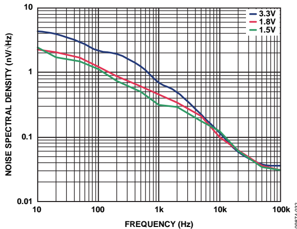
Figure 32. Output Noise Spectral Density, V_{IN} = 5\text{ V} , I_{LOAD} = 10\text{ mA}
