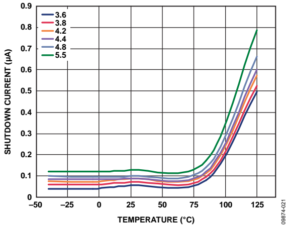
Figure 21. Shutdown Current vs. Temperature at Various Input Voltages
