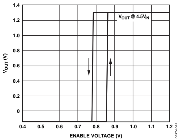
Figure 44. Typical EN_x Pin Operation
