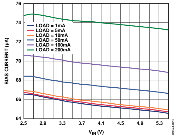
Figure 20. Bias Current vs. Input Voltage, Single Output Load
