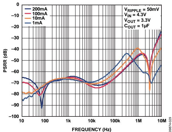
Figure 29. Power Supply Rejection Ratio vs. Frequency, 3.3 V
