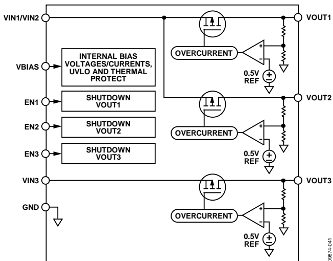
Figure 41. Internal Block Diagram
