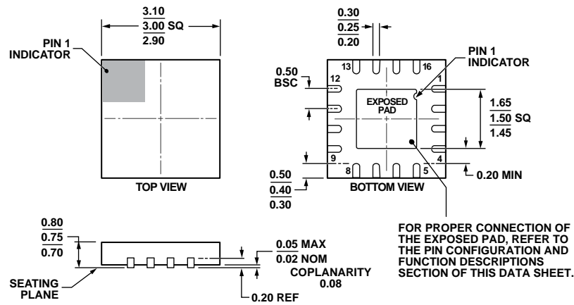
Figure 53. 16-Lead Lead Frame Chip Scale Package [LFCSP_WQ] 3 mm × 3 mm Body, Very, Very Thin Quad (CP-16-27) Dimensions shown in millimeters
