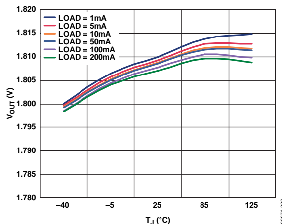
Figure 6. Output Voltage vs. Junction Temperature
