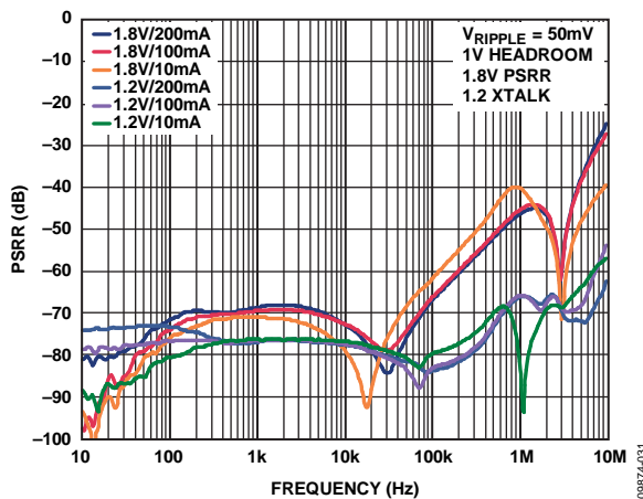
Figure 31. Power Supply Rejection Ratio vs. Frequency, Channel to Channel Crosstalk
