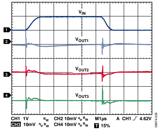
Figure 38. Line Transient Response, V_{IN} = 4\text{ V to } 5\text{ V} , I_{LOAD1} = I_{LOAD2} = I_{LOAD3} = 100\text{ mA} , CH1 = V_{IN} , CH2 = V_{OUT1} , CH3 = V_{OUT2} , CH4 = V_{OUT3}
