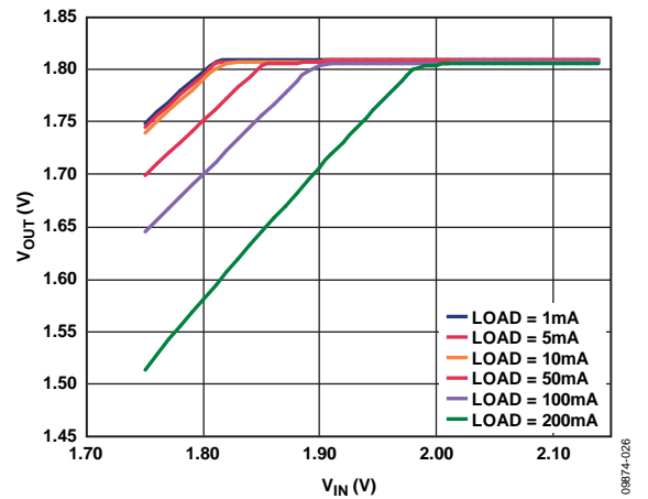
Figure 26. Output Voltage vs. Input Voltage (in Dropout), V_{OUT2} = 1.8\text{ V}
