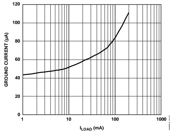
Figure 13. Ground Current vs. Load Current, Single Output Loaded
