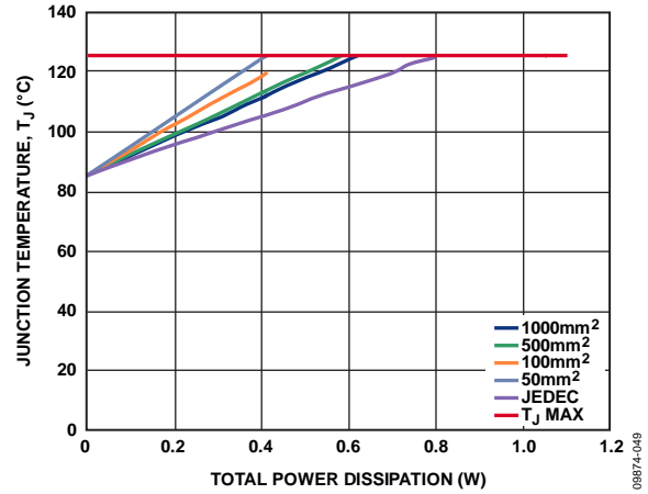
Figure 49. Junction Temperature vs. Total Power Dissipation, T_A = 85^\circ\text{C}
