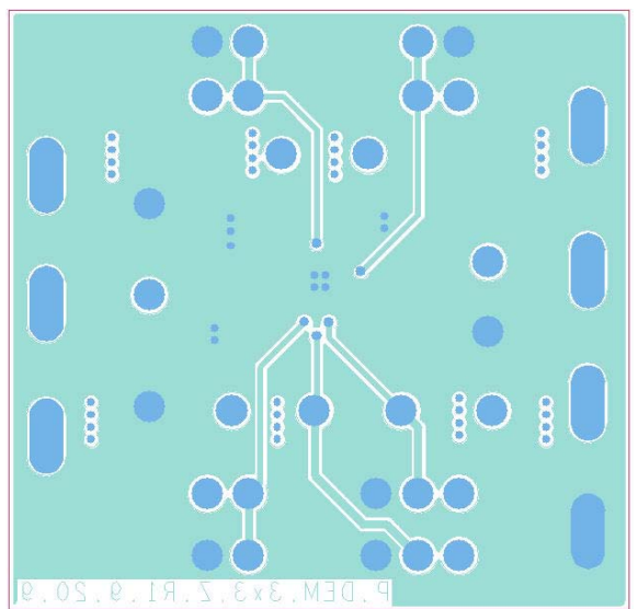
Figure 52. Example of PCB Layout, Bottom Side
