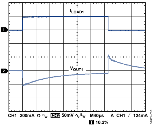
Figure 35. Load Transient Response, I_{LOAD1} = 1\text{ mA to } 200\text{ mA} , C_{OUT1} = 1\text{ }\mu\text{F} , CH1 = I_{LOAD1} , CH2 = V_{OUT1}
