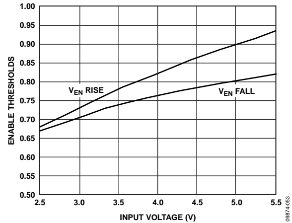
Figure 45. Typical EN_x Pins Thresholds vs. Input Voltage
