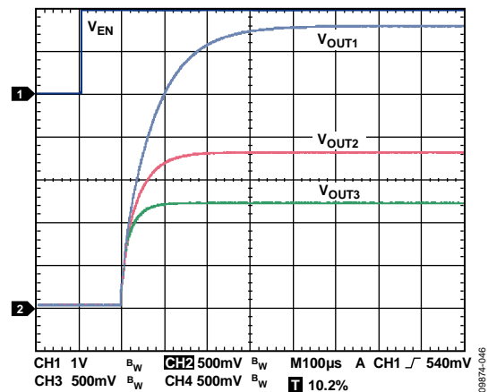
Figure 46. Typical Start-Up Time, I_{LOAD1} = I_{LOAD2} = I_{LOAD3} = 100 \text{ mA} , CH1 = V_{EN} , CH2 = V_{OUT1} , CH3 = V_{OUT2} , CH4 = V_{OUT3}
