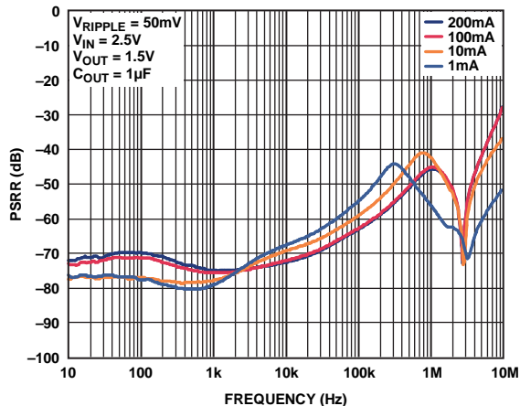
Figure 30. Power Supply Rejection Ratio vs. Frequency, 1.5 V
