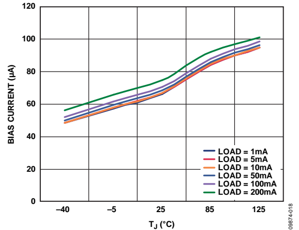
Figure 18. Bias Current vs. Junction Temperature, Single Output Loaded
