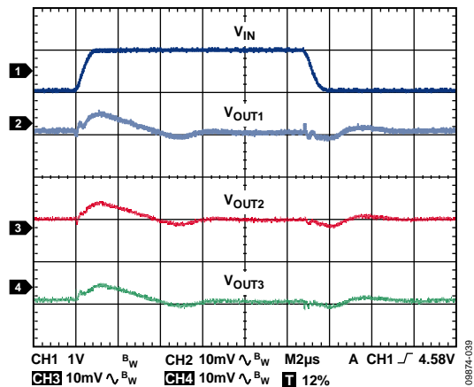
Figure 39. Line Transient Response, V_{IN} = 4V to 5V , I_{LOAD1} = I_{LOAD2} = I_{LOAD3} = 1mA , CH1 = V_{IN} , CH2 = V_{OUT1} , CH3 = V_{OUT2} , CH4 = V_{OUT3}
