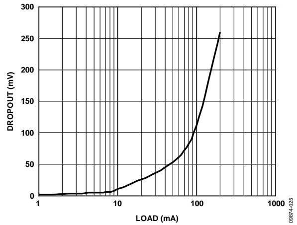
Figure 25. Dropout Voltage vs. Load Current and Output Voltage, V_{OUT2} = 1.8\text{ V}
