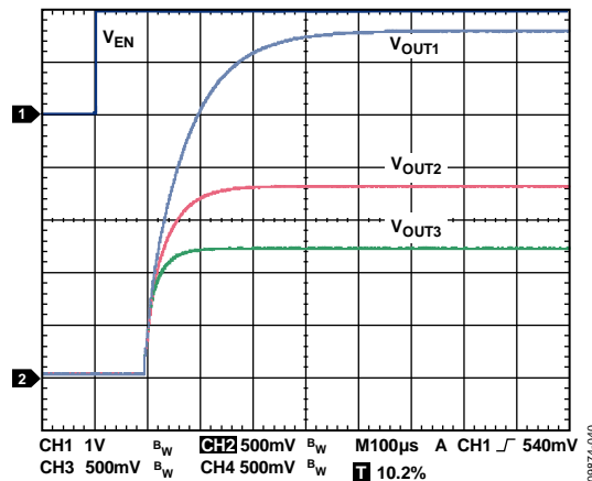
Figure 40. Turn On Response, I_{LOAD1} = I_{LOAD2} = I_{LOAD3} = 100mA , CH1 = V_{EN} , CH2 = V_{OUT1} , CH3 = V_{OUT2} , CH4 = V_{OUT3}
