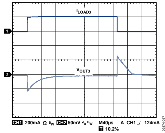
Figure 37. Load Transient Response, I_{LOAD3} = 1\text{ mA to } 200\text{ mA} , C_{OUT3} = 1\text{ }\mu\text{F} , CH1 = I_{LOAD3} , CH2 = V_{OUT3}
