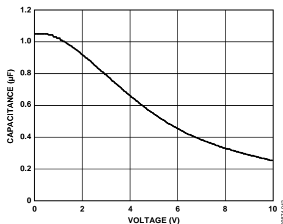
Figure 43. Capacitance vs. Voltage Bias Characteristic
