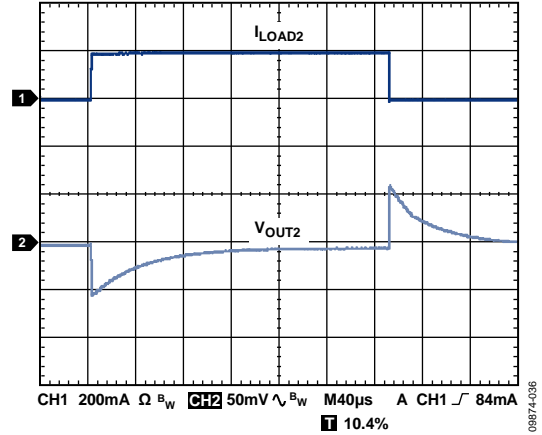
Figure 36. Load Transient Response, I_{LOAD2} = 1\text{ mA to } 200\text{ mA} , C_{OUT2} = 1\text{ }\mu\text{F} , CH1 = I_{LOAD2} , CH2 = V_{OUT2}
