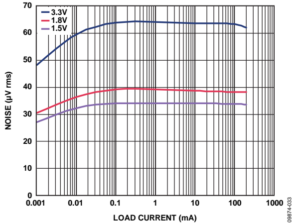
Figure 33. Output Noise vs. Load Current and Output Voltage, V_{IN} = 5V
