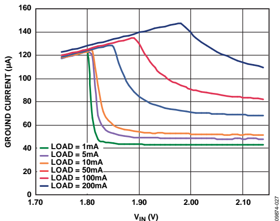
Figure 27. Ground Current vs. Input Voltage in Dropout, V_{OUT2} = 1.8\text{ V}
