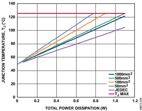
Figure 48. Junction Temperature vs. Total Power Dissipation, T_A = 50^\circ\text{C}
