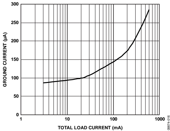
Figure 16. Ground Current vs. Load Current, All Outputs Loaded Equally
