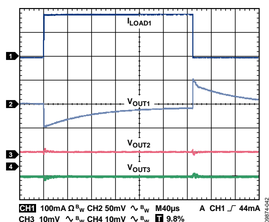
Figure 42. Output Transient Response, I_{LOAD1} = 1\ \text{mA} to 200\ \text{mA} , I_{LOAD2} = 1\ \text{mA} , I_{LOAD3} = 1\ \text{mA} , CH1 = I_{LOAD1} , CH2 = V_{OUT1} , CH3 = V_{OUT2} , CH4 = V_{OUT3}
