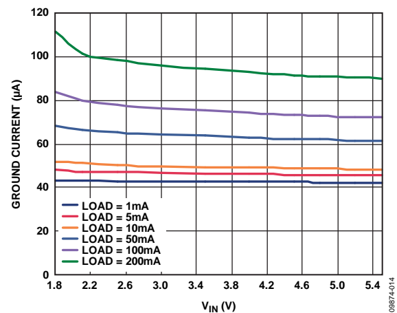
Figure 14. Ground Current vs. Input Voltage, Single Output Loaded
