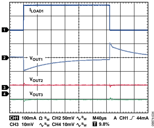
Figure 34. Load Transient Response, I_{LOAD1} = 1\text{ mA to } 200\text{ mA} , I_{LOAD2} = I_{LOAD3} = 1\text{ mA} , CH1 = I_{LOAD1} , CH2 = V_{OUT1} , CH3 = V_{OUT2} , CH4 = V_{OUT3}
