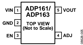
Figure 5. 5-Lead TSOT, Adjustable Output Pin Configuration, ADP161/ADP163
