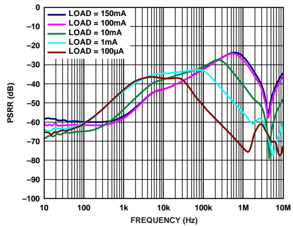
Figure 23. Adjustable ADP161 Power Supply Rejection Ratio vs. Frequency, V_{OUT} = 3.3V , V_{IN} = 4.3V
