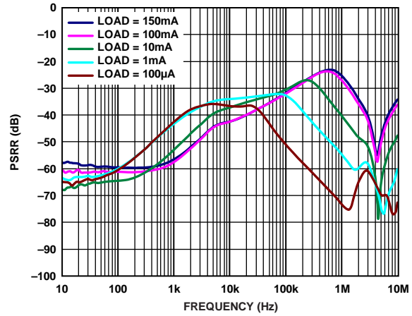
Figure 22. Power Supply Rejection Ratio vs. Frequency Various Output Voltages and Load Currents, V_{OUT} = 3.3V , V_{IN} = 3.8V
