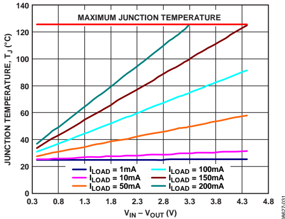
Figure 39. WLCSP 500 mm² of PCB Copper, T_A = 25^\circ\text{C}
