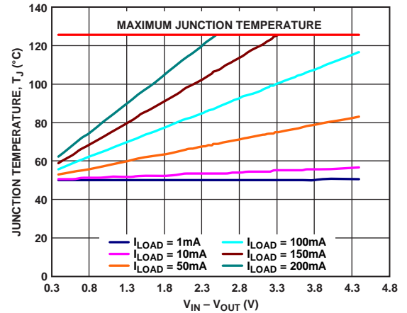
Figure 42. WLCSP 500 mm² of PCB Copper, T_A = 50^\circ\text{C}
