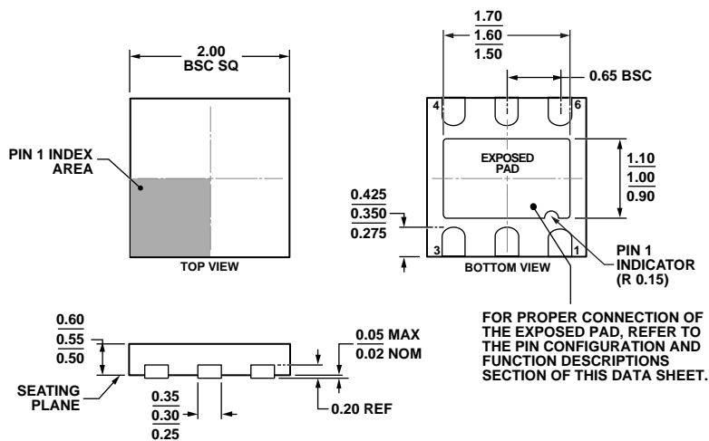
Figure 65. 6-Lead Lead Frame Chip Scale Package [LFCSF_UD] 2.00 mm x 2.00 mm Body, Ultra Thin, Dual Lead (CP-6-3)
