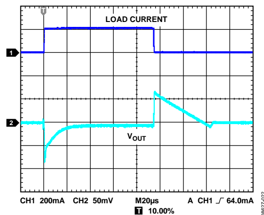
Figure 24. Load Transient Response, C_{IN} = 1\text{ μF} , C_{OUT} = 1\text{ μF} , I_{LOAD} = 1\text{ mA} to 200\text{ mA}
