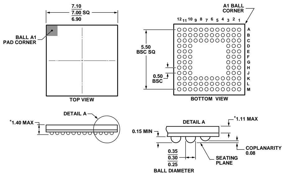
*COMPLIANT WITH JEDEC STANDARDS MO-195-BD WITH EXCEPTION TO PACKAGE HEIGHT AND THICKNESS. Figure 40. 108-Ball Chip Scale Package Ball Grid Array [CSP_BGA] (BC-108-4) Dimensions shown in millimeters
