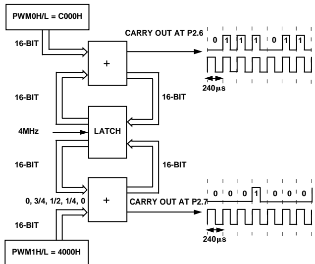
Figure 62. PWM Mode 6
