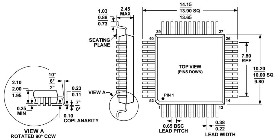
Figure 95. 52-Lead Metric Quad Flat Package [MQFP] (S-52-2)
