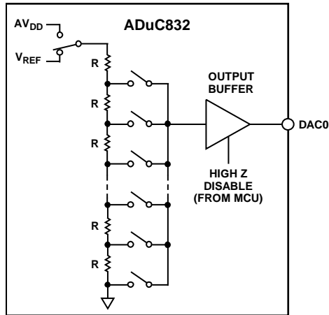
Figure 51. Resistor String DAC Functional Equivalent
