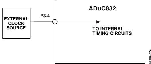
Figure 86. Connecting an External Clock Source
