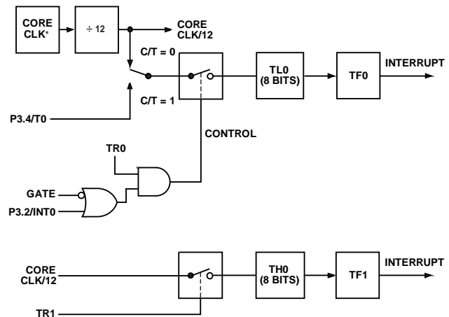
Figure 78. Timer/Counter 0, Mode 3
