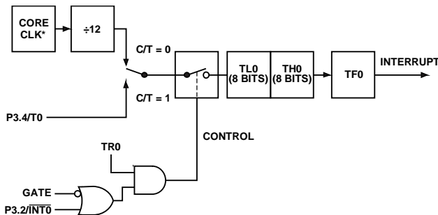
Figure 76. Timer/Counter 0, Mode 1
