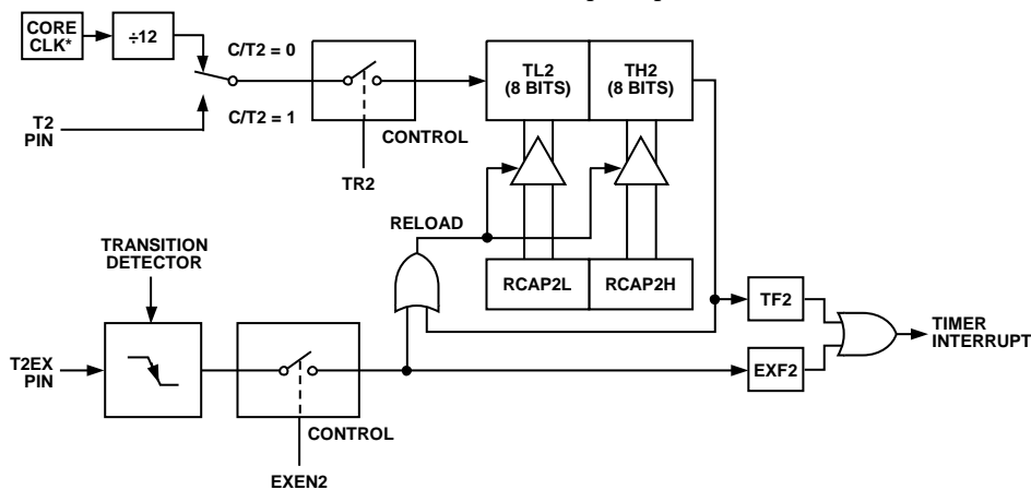
Figure 79. Timer/Counter 2, 16-Bit Autoreload Mode
