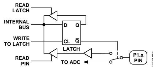
Figure 67. Port 1 Bit Latch and I/O Buffer
