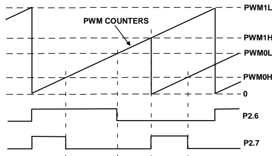
Figure 61. PWM Mode 5
