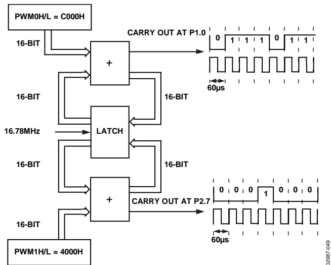
Figure 60. PWM Mode 4
