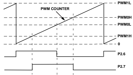
Figure 58. PWM Mode 2
