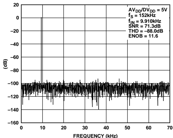
Figure 26. Dynamic Performance at V_{DD} = 5V
