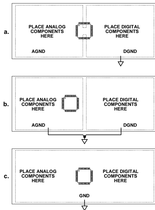
Figure 93. System Grounding Schemes
