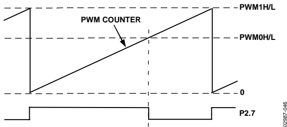
Figure 57. PWM Mode 1
