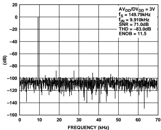
Figure 27. Dynamic Performance at V_{DD} = 3V
