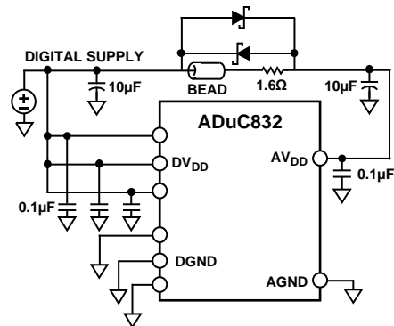
Figure 91. External Single-Supply Connections
