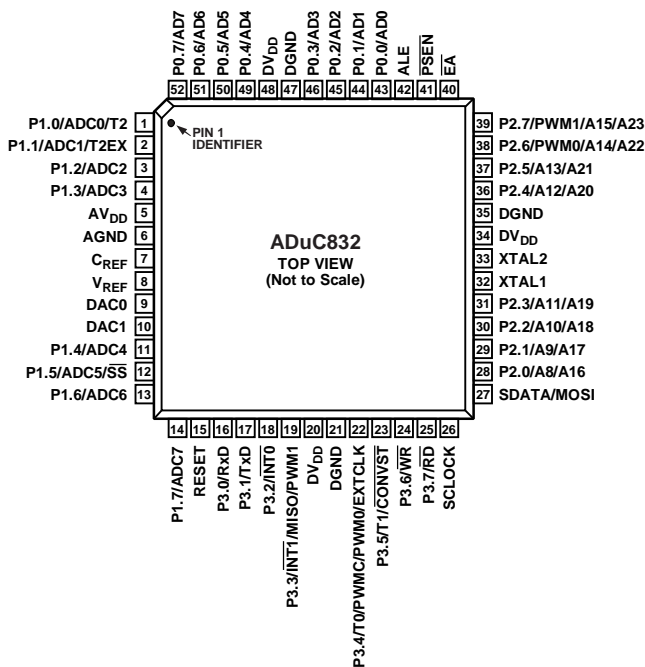
Figure 14. 52-Lead MQFP
