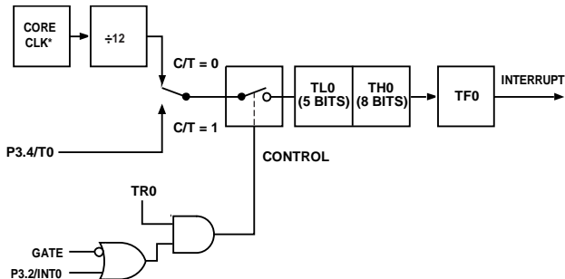
Figure 75. Timer/Counter 0, Mode 0
