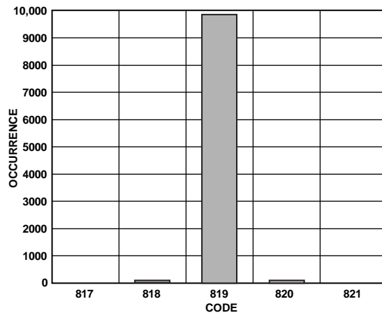
Figure 25. Code Histogram Plot, V_{DD} = 3V
