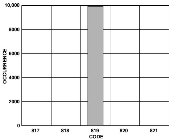
Figure 24. Code Histogram Plot, V_{DD} = 5V
