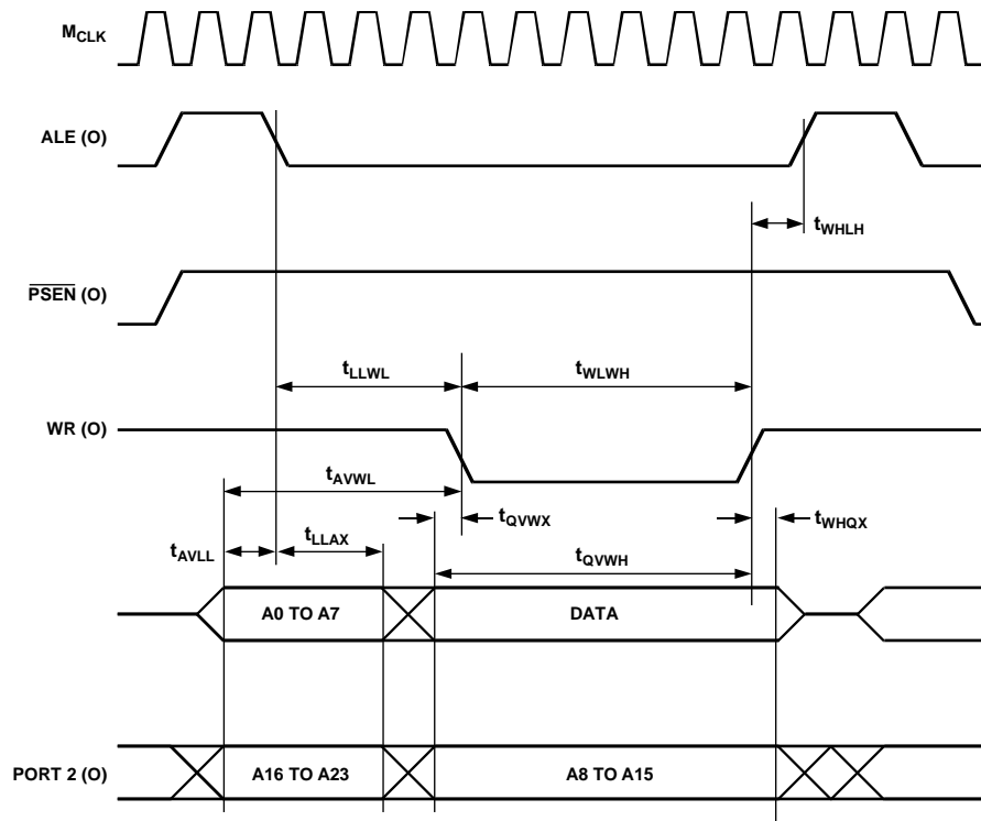
Figure 7. External Data Memory Write Cycle
