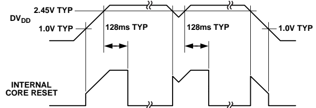
Figure 92. Internal POR Operation
