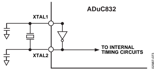
Figure 85. External Parallel Resonant Crystal Connections
