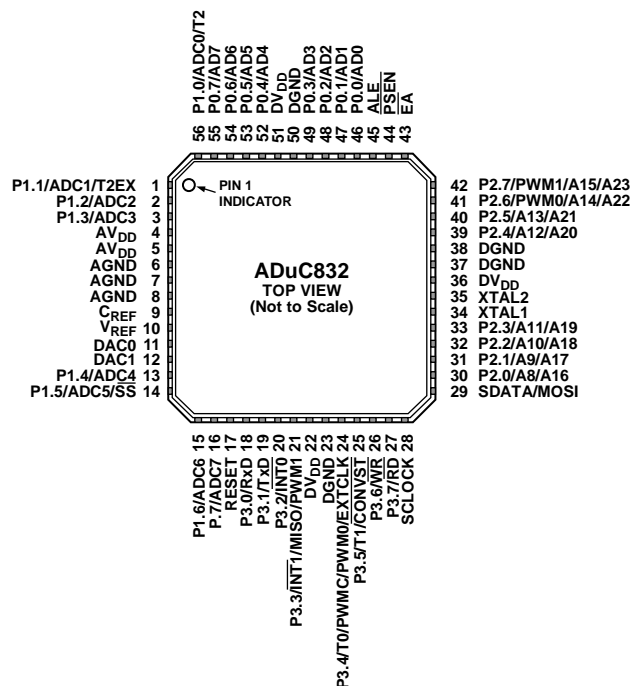
Figure 15. 56-Lead LFCSP
