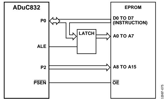
Figure 87. External Program Memory Interface
