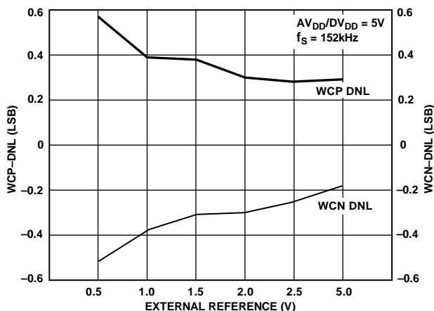
Figure 22. Typical Worst-Case DNL Error vs. V_{REF} , V_{DD} = 5V
