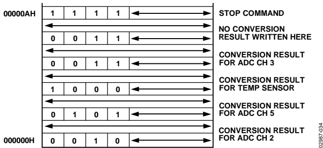
Figure 45. Typical External Memory Configuration Post-ADC DMA Operation
