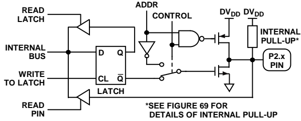
Figure 68. Port 2 Bit Latch and I/O Buffer
