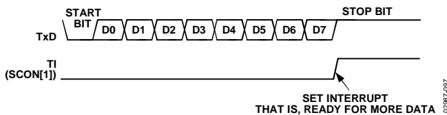
Figure 82. UART Serial Port Transmission, Mode 0
