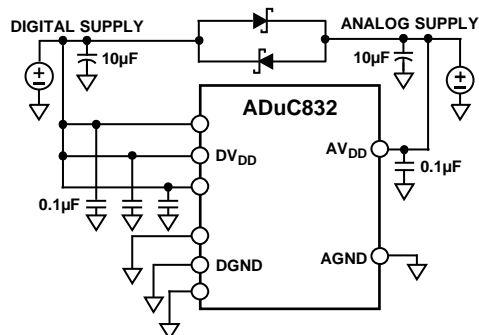
Figure 90. External Dual-Supply Connections
