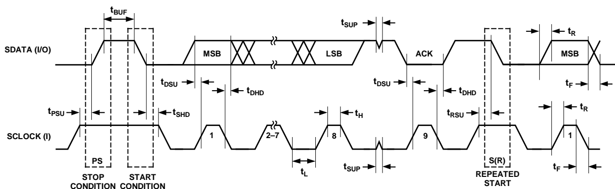
Figure 9. I 2 C Compatible Interface Timing
