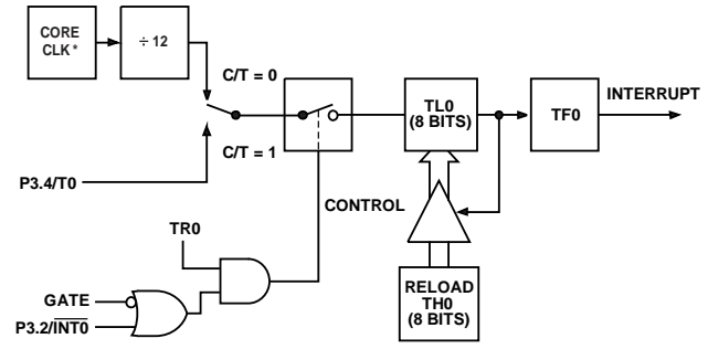
Figure 77. Timer/Counter 0, Mode 2
