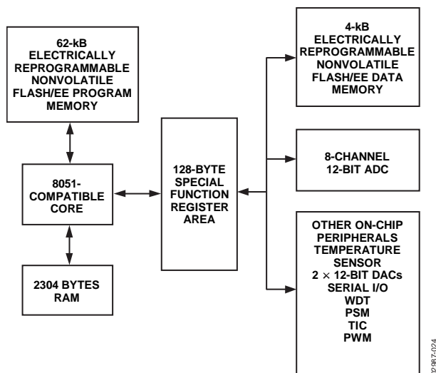
Figure 35. Programming Model
