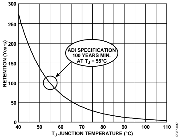
Figure 48. Flash/EE Memory Data Retention
