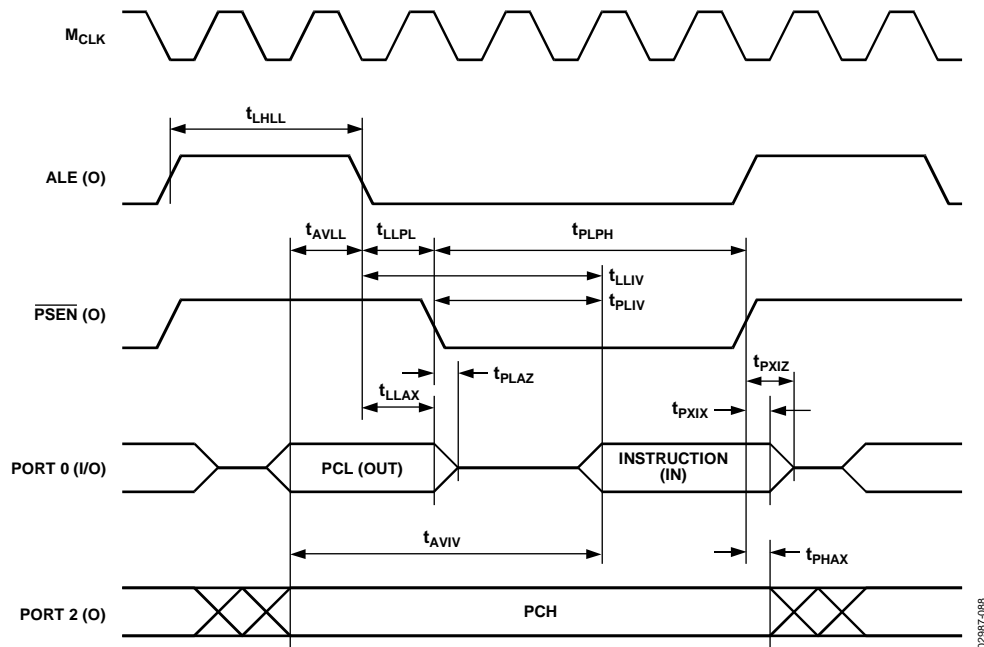
Figure 5. External Program Memory Read Cycle
