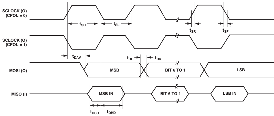
Figure 10. SPI Master Mode Timing (CPHA = 1)
