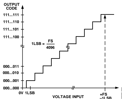
Figure 37. ADC Transfer Function
