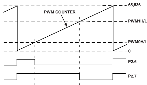
Figure 59. PWM Mode 3
