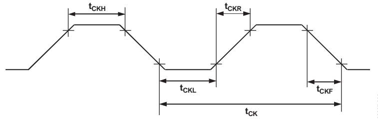
Figure 3. XTAL1 Input
