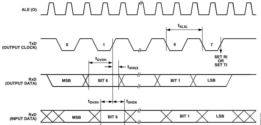
Figure 8. UART Timing in Shift Register Mode
