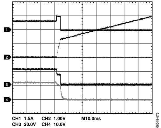
Figure 47. Overcurrent Condition During Operation (ADM1178-1 Model) (Channel 1 = I_{LOAD} , Channel 2 = V_{TIMER} , Channel 3 = V_{GATE} , Channel 4 = V_{OUT} )
