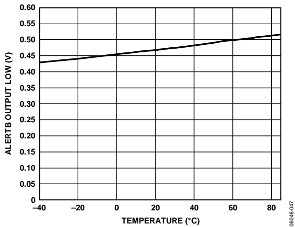
Figure 30. ALERTB Output Low Voltage vs. Temperature @ 1 mA
