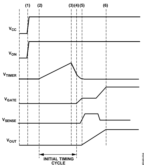
Figure 33. Startup (ON Asserts as Power Is Applied)
