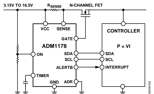
Figure 2. Applications Diagram
