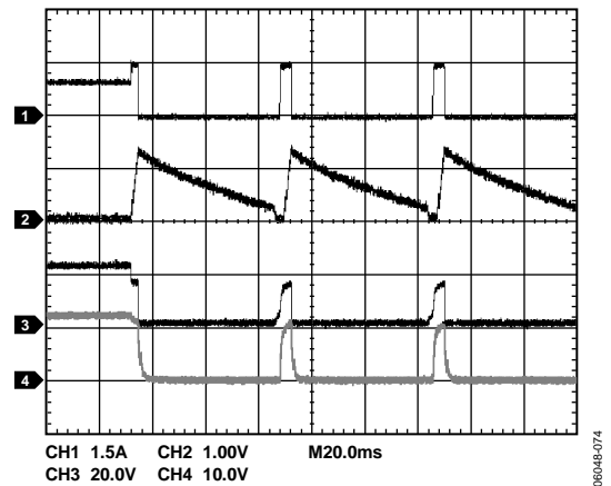
Figure 48. Overcurrent Condition During Operation (ADM1178-2 Model) (Channel 1 = I_{LOAD} , Channel 2 = V_{TIMER} , Channel 3 = V_{GATE} , Channel 4 = V_{OUT} )
