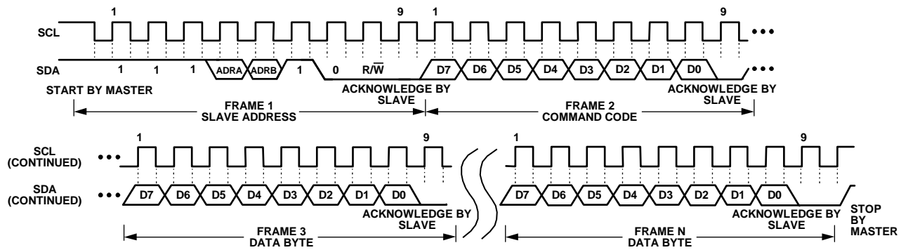
Figure 35. General I2C Write Timing Diagram
