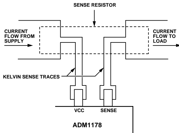
Figure 50. Kelvin Sense Connections
