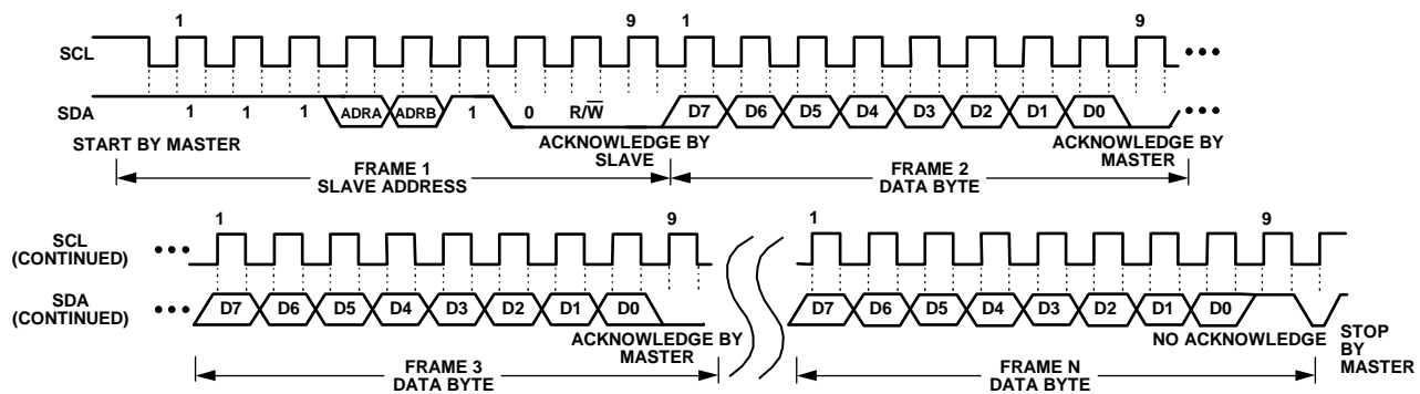
Figure 36. General I2C Read Timing Diagram
