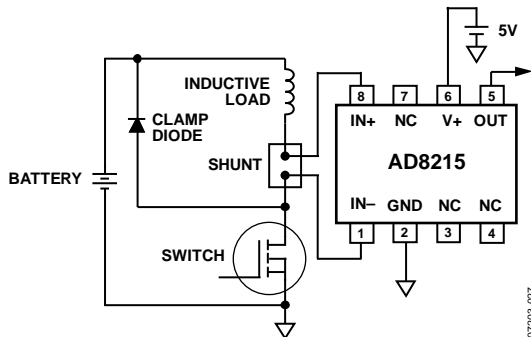
Figure 28. Low-Side Switch
