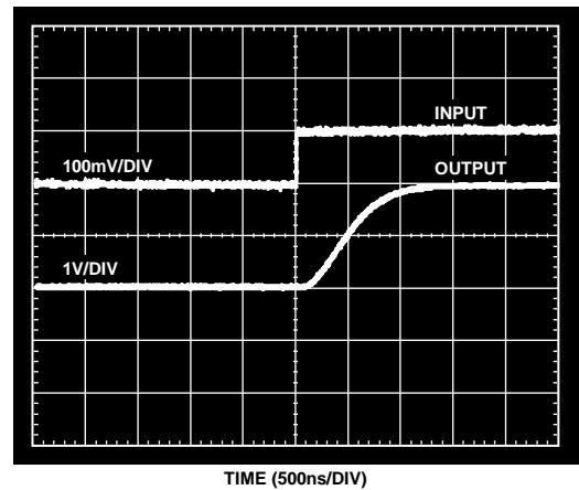
Figure 14. Rise Time
