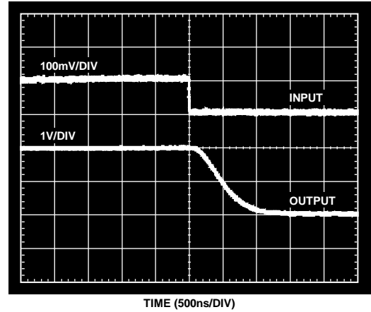
Figure 13. Fall Time
