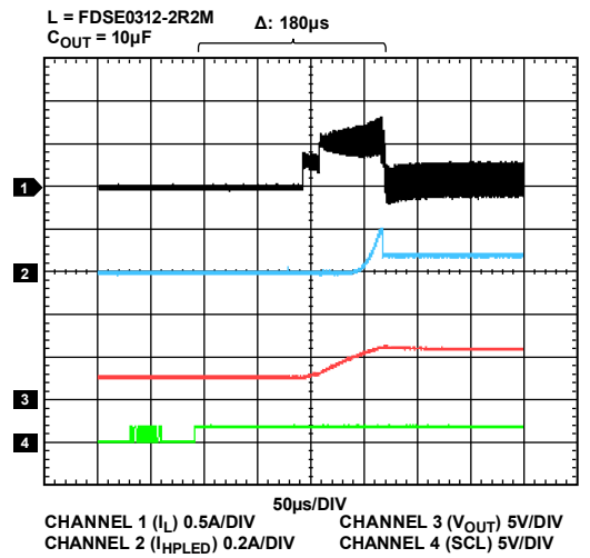
Figure 9. Startup, Two LEDs Assist Light Mode, I LED = 40 mA, V IN = 3.2 V
