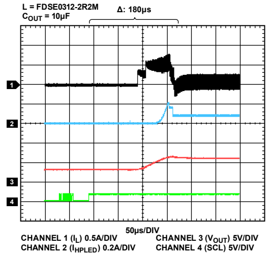
Figure 10. Startup, Two LEDs Torch Mode, I LED = 40 mA, V IN = 3.6 V
