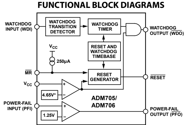
* VOLTAGE REFERENCE = 4.65V (ADM705), 4.40V (ADM706)
