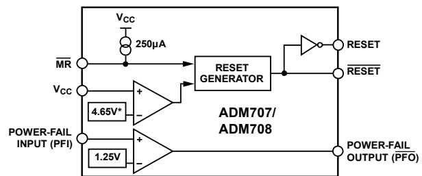
* VOLTAGE REFERENCE = 4.65V (ADM707), 4.40V (ADM708)
