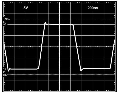
Figure 42. Large Signal Pulse Response of the Inverting Amplifier Using Current Feedback Compensation, C_{COMP} = 1 \text{ pF} , R_F = 3 \text{ k}\Omega , R_1 = 3 \text{ k}\Omega
