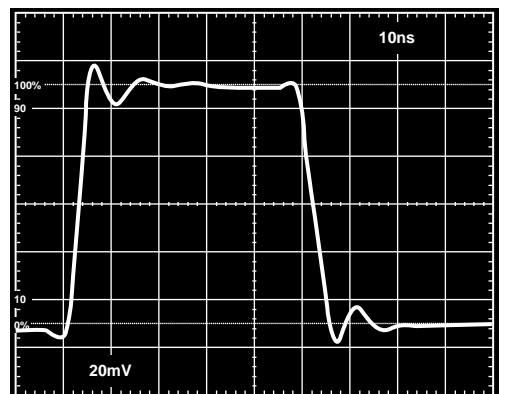
Figure 43. Small Signal Pulse Response of Inverting Amplified Using Current Feedback Compensation, C_{COMP} = 4 \text{ pF} , R_F = 1 \text{ k}\Omega , R_1 = 1 \text{ k}\Omega
