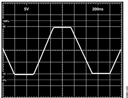
Figure 40. Large Signal Pulse Response of Inverting Amplifier Using Current Feedback Compensation, C_{COMP} = 15 \text{ pF} , C_1 = 15 \text{ pF} , R_F = 1 \text{ k}\Omega , R_1 = 1 \text{ k}\Omega
