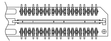
DIFFERENTIAL PAIR LOADING (BOTTOM VIEW) SCALE 2:1
