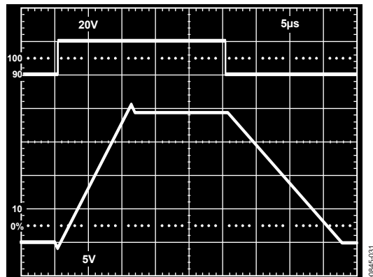
Figure 31. Unity Gain Follower Large Signal Pulse Response
