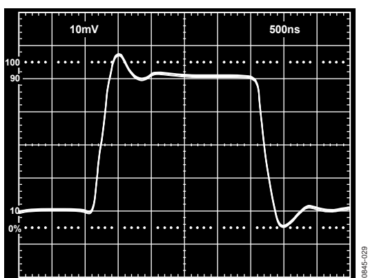
Figure 29. Unity Gain Inverter Small Signal Pulse Response
