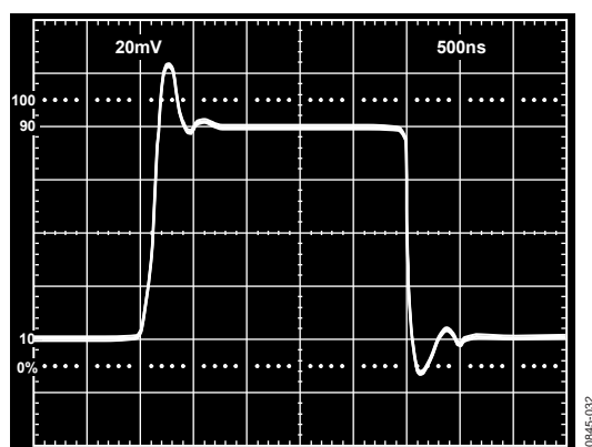
Figure 32. Unity Gain Follower Small Signal Pulse Response
