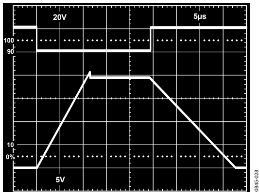
Figure 28. Unity Gain Inverter Large Signal Pulse Response
