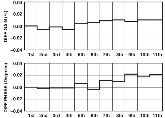
TPC 33. AD8048 Differential Gain and Phase Error, G = +2 , R_L = 150 \Omega , R_F = 200 \Omega , R_{IN} = 200 \Omega
