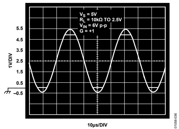
Figure 36. Output Voltage
