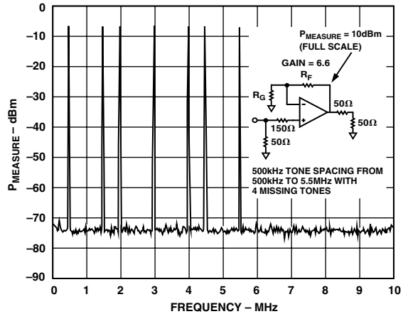
Figure 12. Multitone Distortion; R_L = 100 \Omega
