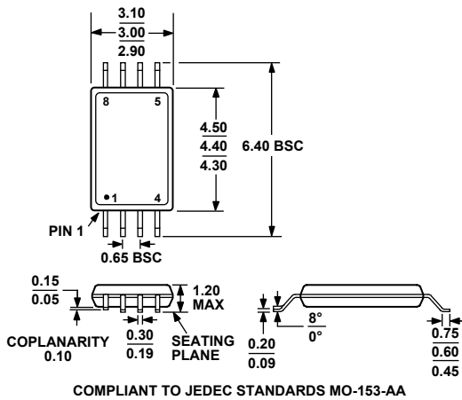
Figure 72. 8-Lead Thin Shrink Small Outline Package [TSSOP] (RU-8) Dimensions shown in millimeters
