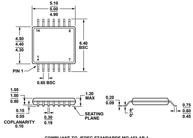
Figure 74. 14-Lead Thin Shrink Small Outline Package [TSSOP] (RU-14) Dimensions shown in millimeters
