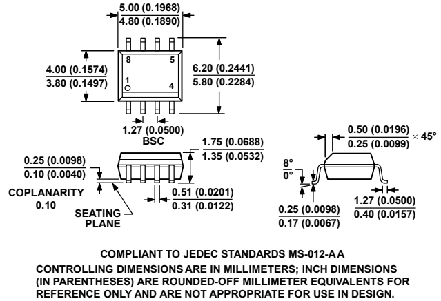
Figure 73. 8-Lead Standard Small Outline Package [SOIC_N] Narrow Body (R-8) Dimensions shown in millimeters and (inches)
