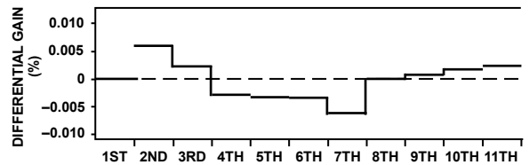
Figure 22. Differential Gain and Phase Error, G = 2 , NTSC Input Signal, R_L = 1k\Omega , V_S = 5V
