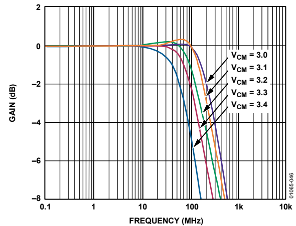
Figure 46. Unity-Gain Follower Bandwidth vs. Input Common Mode, V_s = 5\text{ V}
