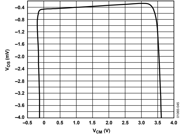
Figure 45. V_{os} vs. Common-Mode Voltage, V_s = 5\text{ V}
