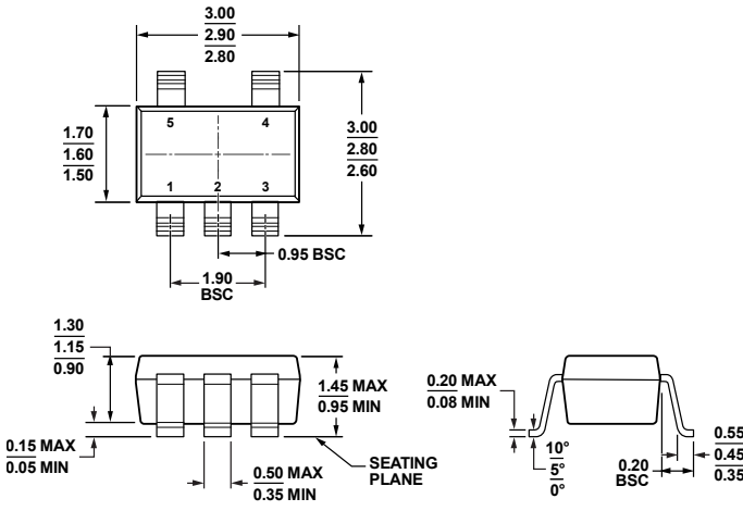
Figure 58. 5-Lead Small Outline Transistor Package [SOT-23] (RJ-5)
