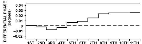
Figure 23. Differential Gain and Phase Error, G = 2 , NTSC Input Signal, R_L = 150\Omega , V_S = 5V
