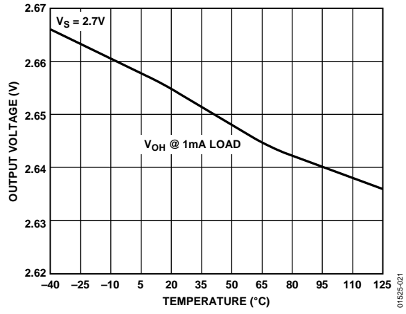
Figure 21. Output Voltage Swing vs. Temperature
