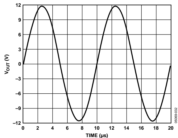
Figure 3. Output Swing, V_S = \pm 12 V, R_L = 100 Ω
