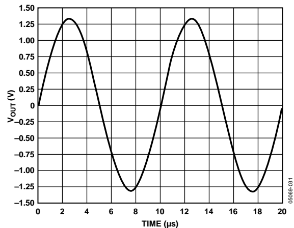
Figure 2. Output Swing, V_S = \pm 1.5 V, R_L = 25 Ω
