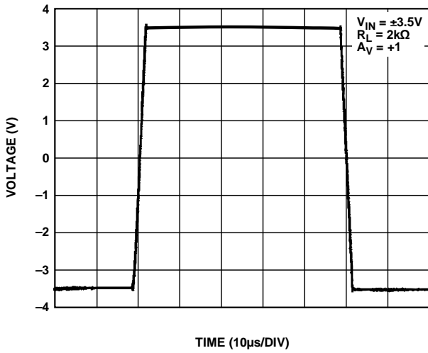
Figure 16. Large-Signal Transient Response, V_{SV} = \pm 5 V
