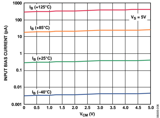
Figure 6. Input Bias Current vs. Common-Mode Voltage
