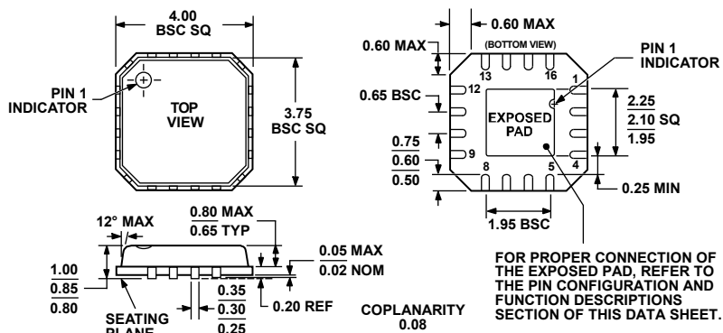
Figure 45.16-Lead Frame Chip Scale Package [LFCSP_VQ] 4 mm × 4 mm Body, Very Thin Quad (CP-16-4)
