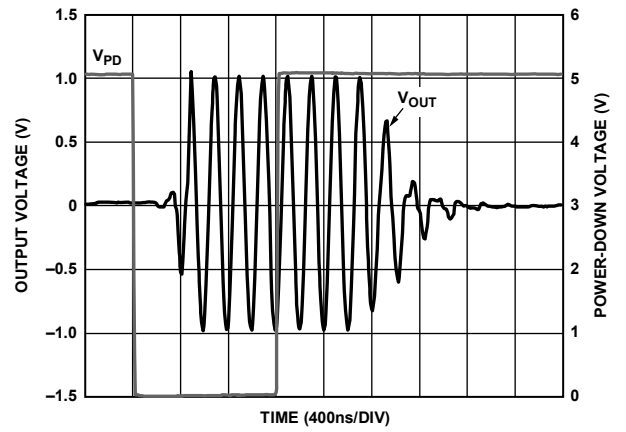
Figure 32. Enable/Power-Down Time
