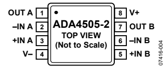
Figure 2. 8-Lead MSOP (RM-8)
