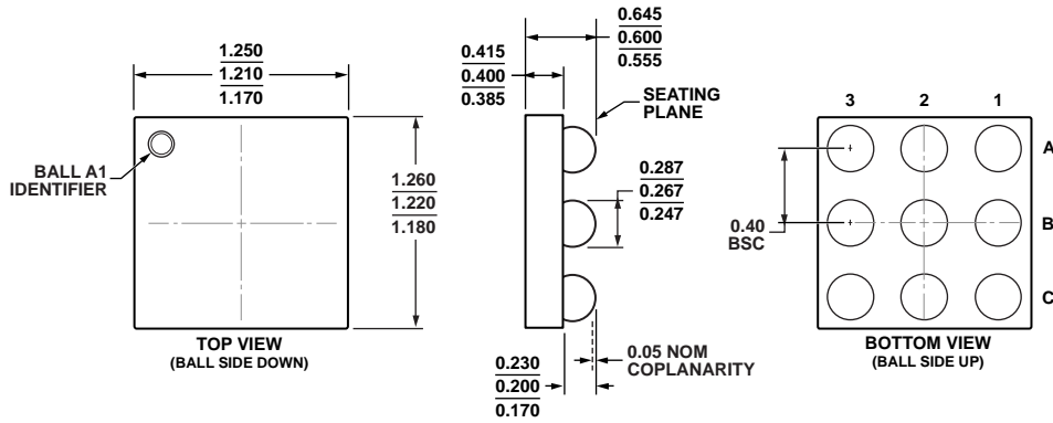
Figure 63. 9-Ball Wafer Level Chip Scale Package [WLCSF] (CB-9-3)
