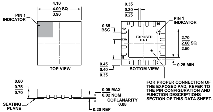
Figure 61. 16-Lead Lead Frame Chip Scale Package [LFCSW_WQ] 4 mm x 4mm Body, Very Very Thin Quad (CP-16-17) Dimensions shown in millimeters
