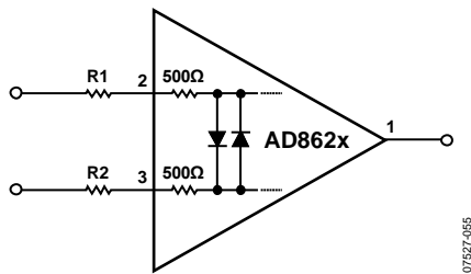
Figure 54. Input Protection
