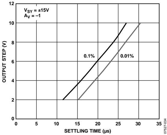
Figure 41. Output Step vs. Settling Time
