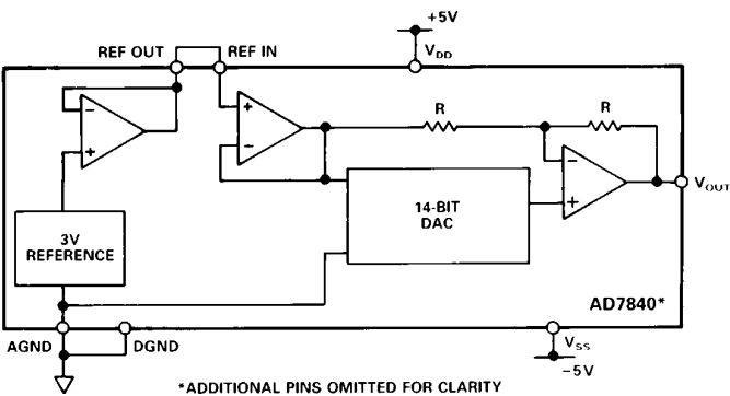
Figure 5. AD7840 Basic Connection Diagram
