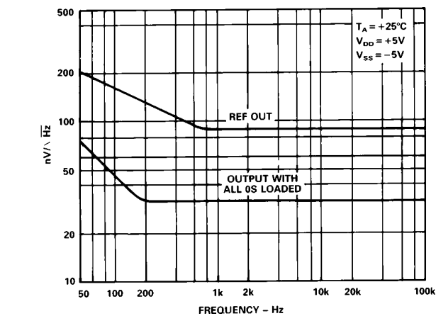
Figure 4. Noise Spectral Density vs. Frequency
