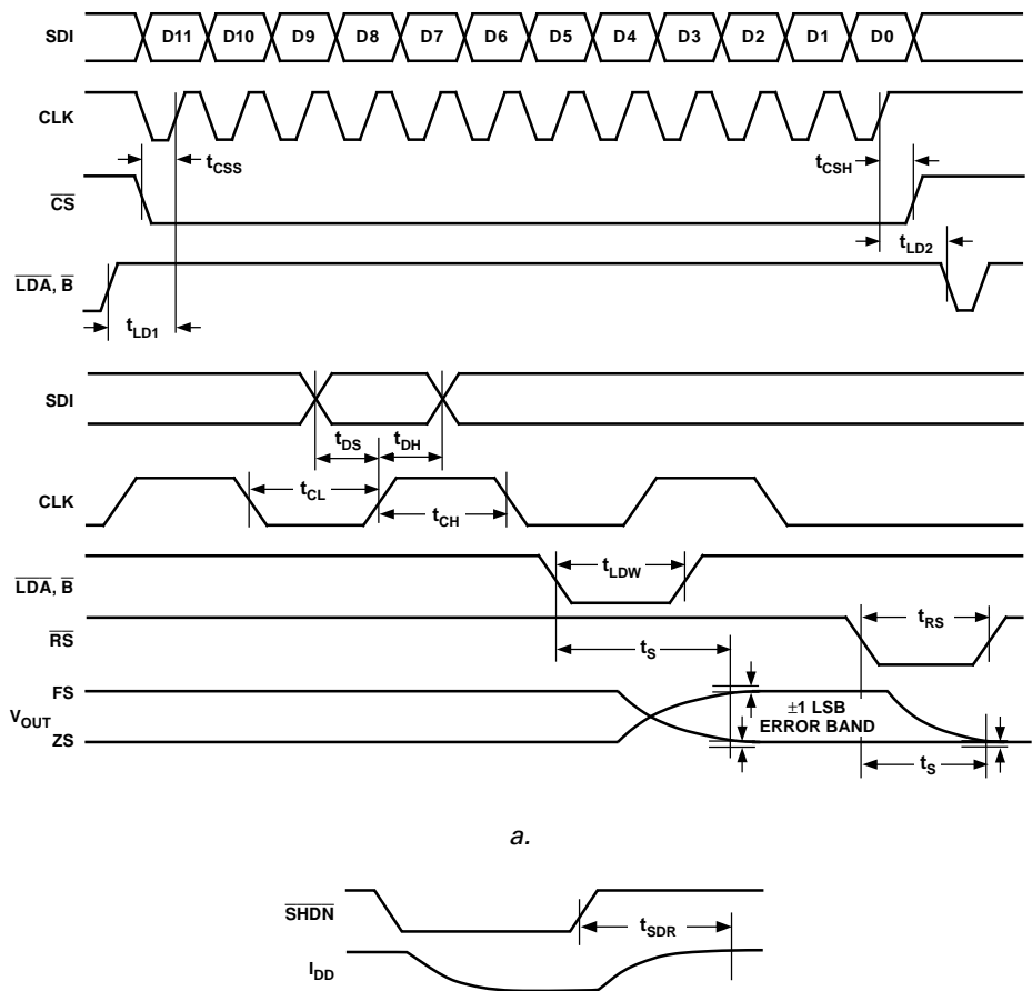
Figure 3. Timing Diagrams
