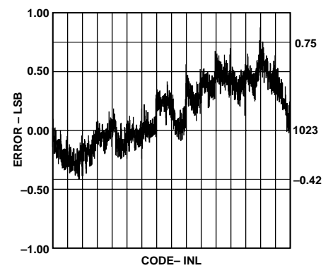
Figure 16. Typical Linearity
