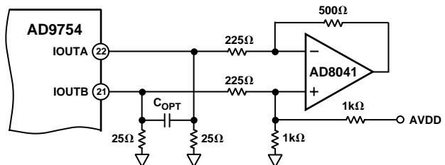
Figure 29. Single-Supply DC Differential Coupled Circuit
