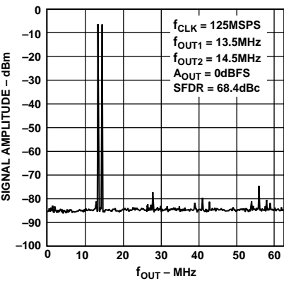
Figure 15. Dual-Tone SFDR
