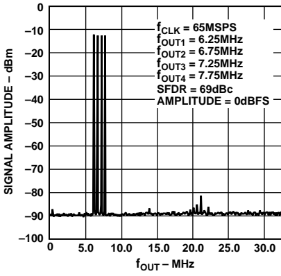
Figure 16. Four-Tone SFDR
