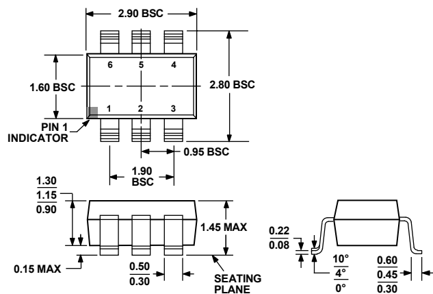
Figure 39. 6-Lead Small Outline Transistor Package [SOT-23] (RJ-6) Dimensions shown in millimeters
