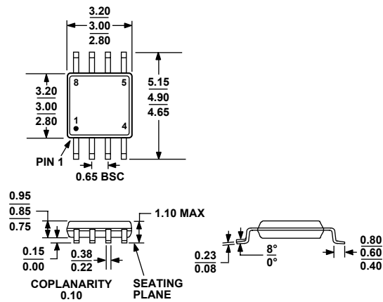
Figure 40. 8-Lead Mini Small Outline Package [MSOP] (RM-8) Dimensions shown in millimeters
