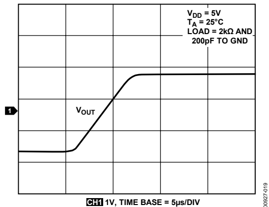
Figure 19. Half-Scale Settling ( 1/4 to 3/4 Scale Code Charge)
